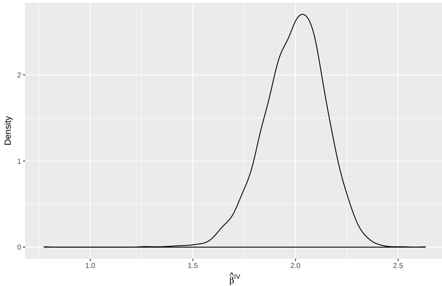
Density of IV Estimator with N = 100 and \rho_{XZ} = .95
